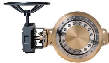
REPLACEABLE SEAT
